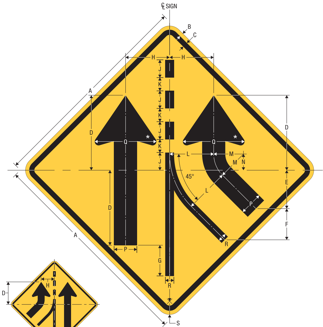
W4-3R ADDED LANE W4-3L
