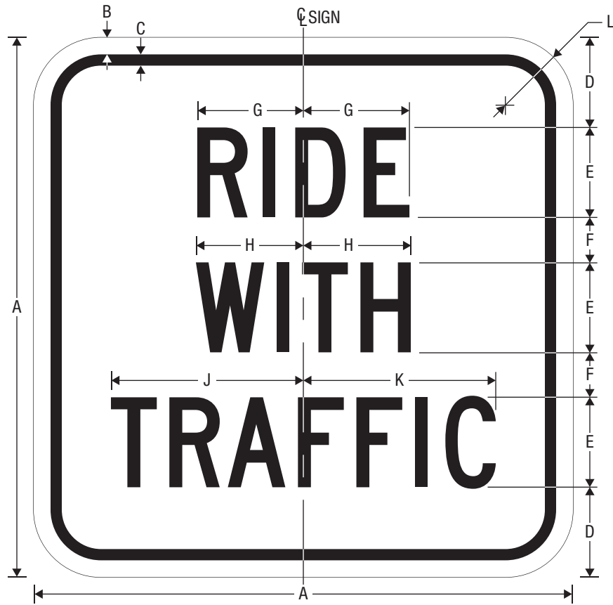
R9-3cP RIDE WITH TRAFFIC (PLAQUE)
