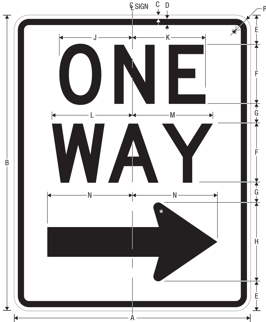
R6-2R ONE WAY
